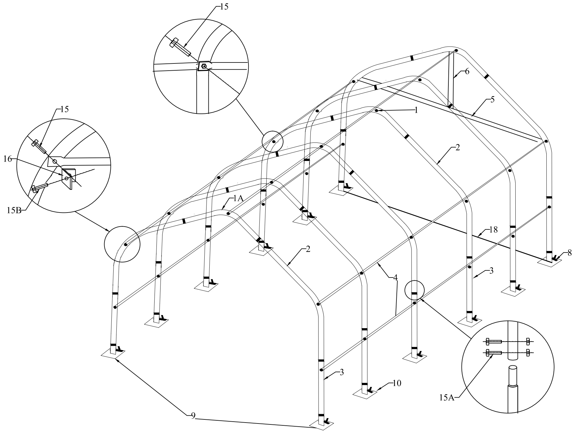
Figure 1: Frame Sketch Size: L10xW3.5xH4.5m
