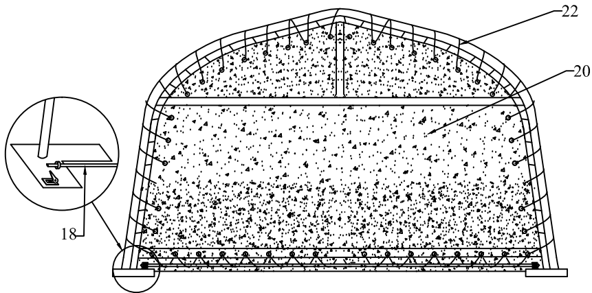
Figure 12 Installation of the Back Cover
