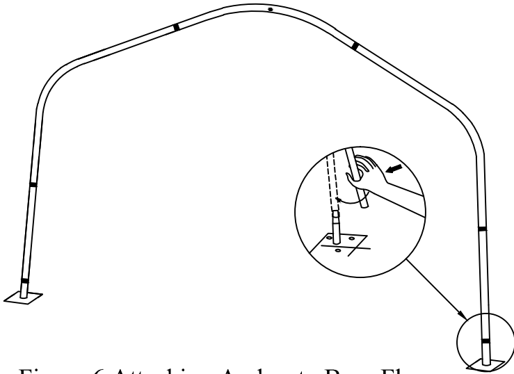
Figure 6 Attaching Arches to Base Flanges
