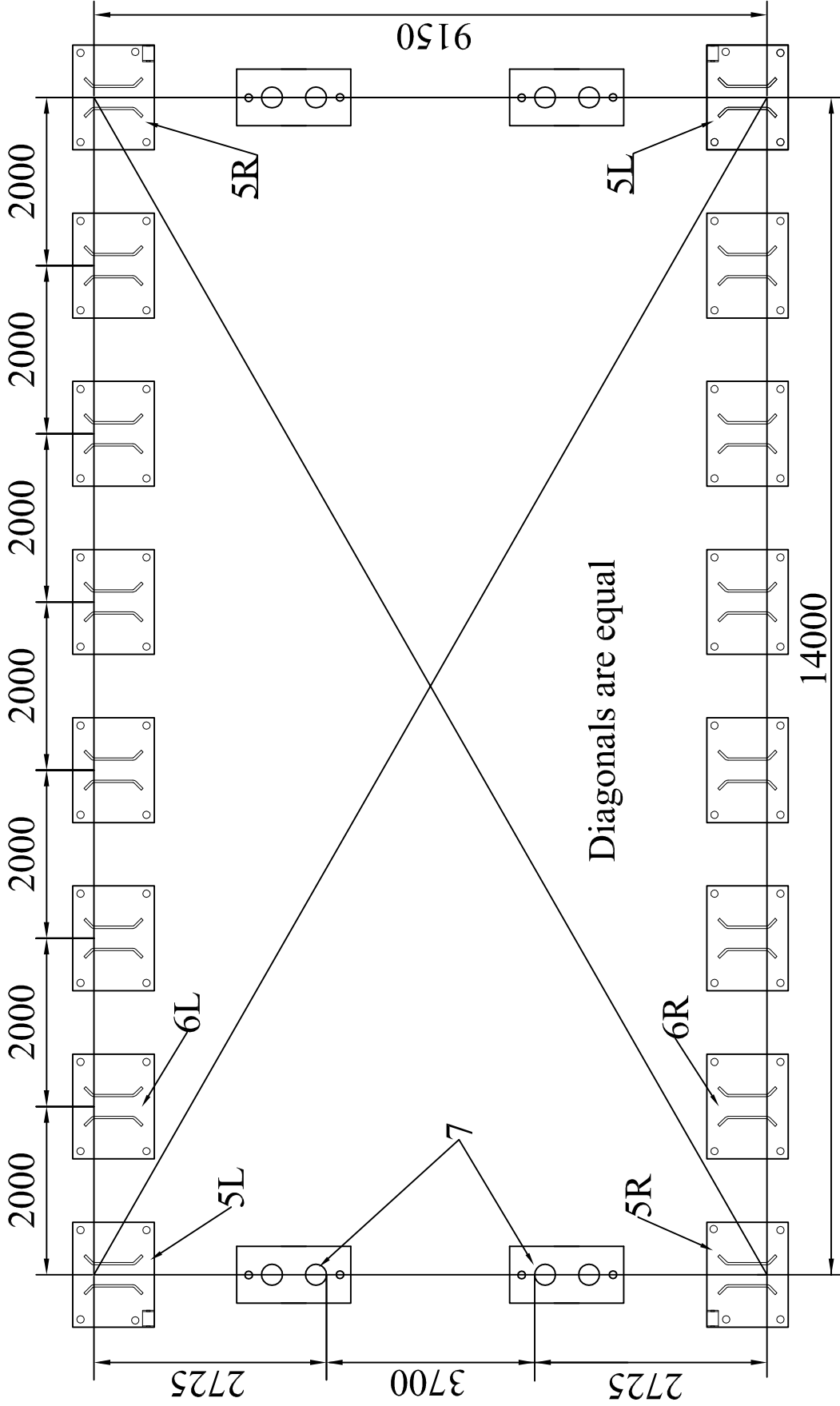
Figure 6 Position of Base Flanges
